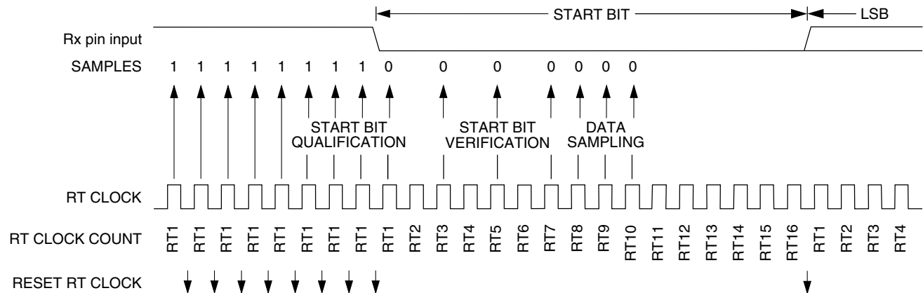
Figure 38-152. Receiver data sampling
