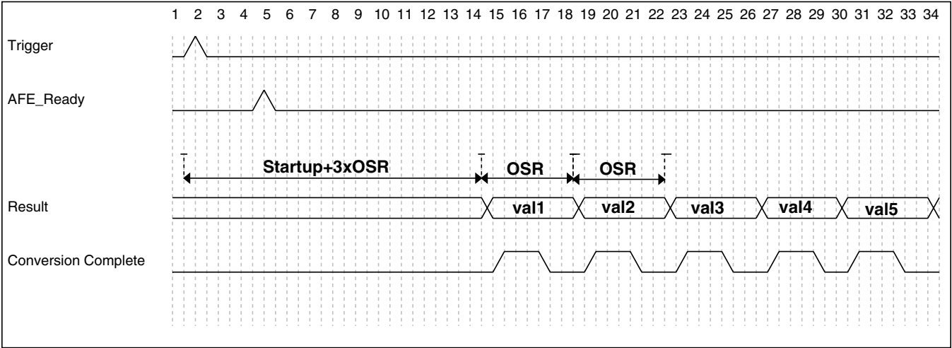
Figure 25-18. Continuous conversion
