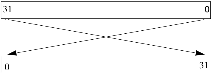
Figure 39-6. Transpose type 10
