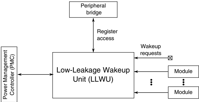
Figure 3-6. Low-Leakage Wake-up Unit configuration
