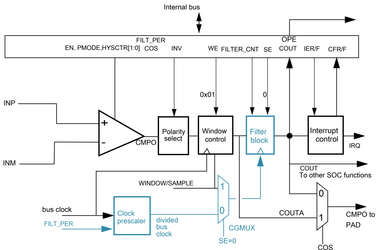
Figure 27-27. Windowed mode
