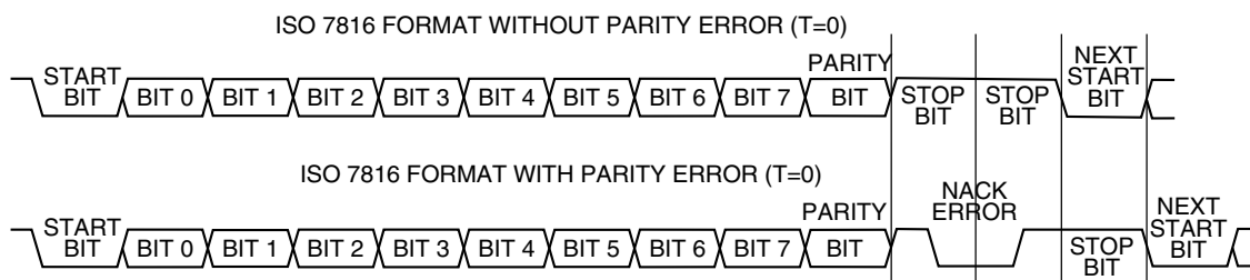
Figure 38-174. ISO-7816 T = 0 data format
