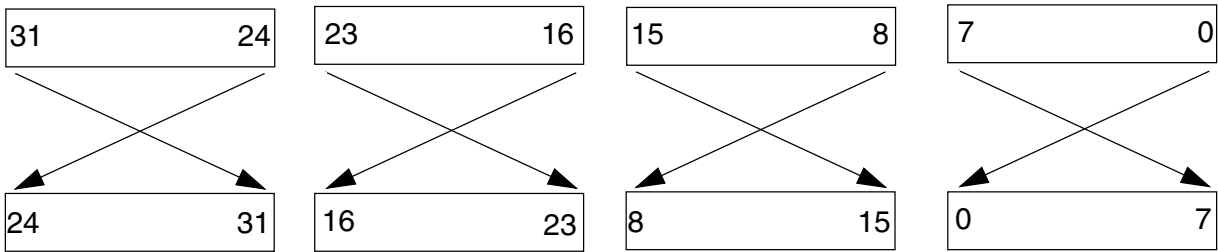
Figure 39-5. Transpose type 01
