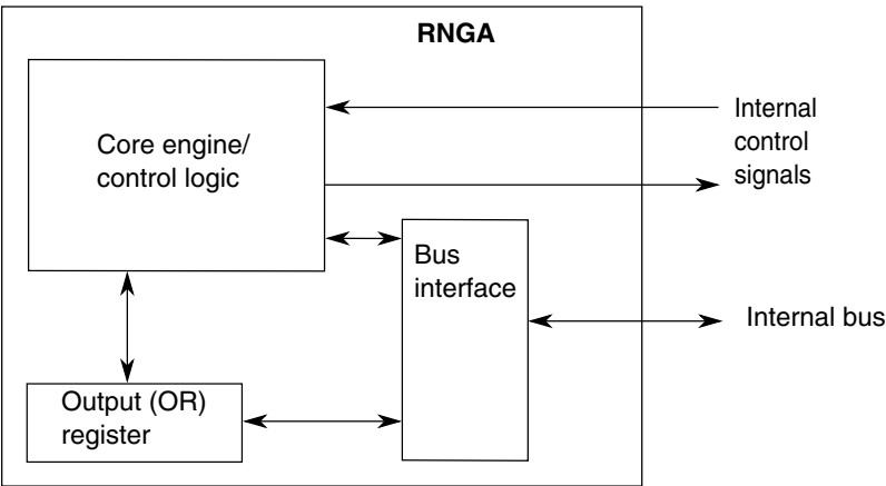
Figure 40-5. RNGA block diagram
