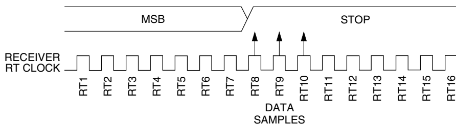
Figure 38-160. Slow data
