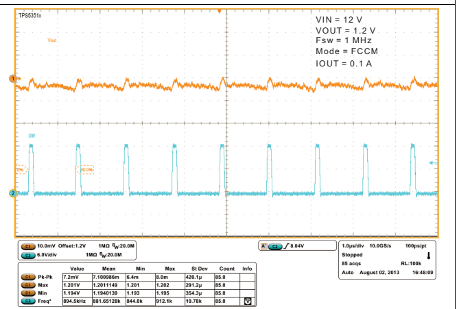
Figure 14. FCCM Steady-State Operation
