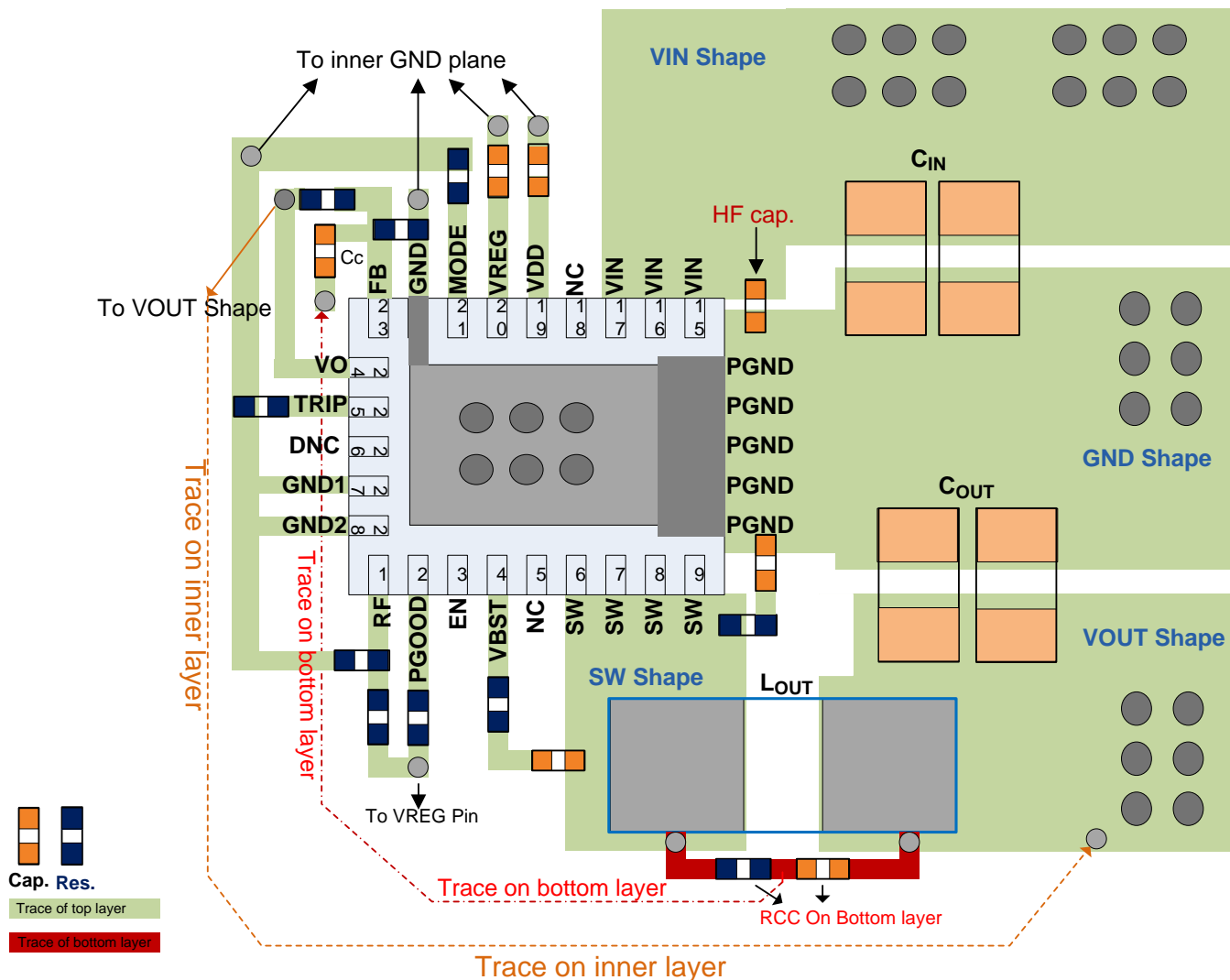
Figure 56. Layout Recommendation
