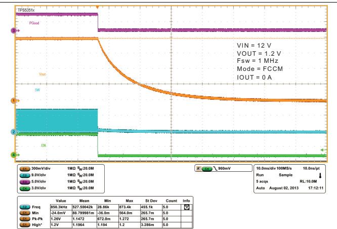
Figure 26. FCCM Shutdown Operation
