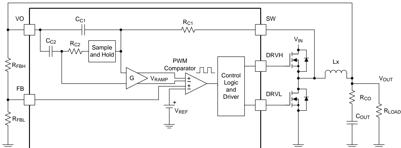
Figure 35. D-CAP3 Mode
