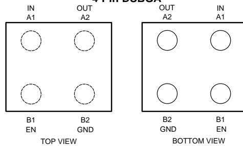
YKE and YKM Packages 4-Pin DSBGA
