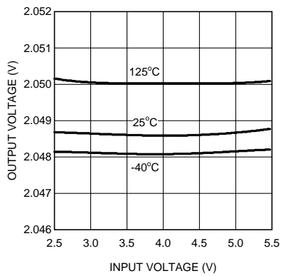
Figure 9. Line Regulation
