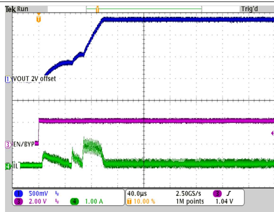
V_{IN} = 2.0V L = 3.3\mu H C_{OUT} = 22 \mu F V_{OUT} = 3.3V VSEL = GND R_{LOAD} = 100\Omega
