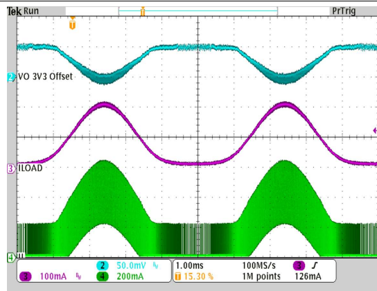
V_{IN} = 1.8V L = 3.3\mu H C_{OUT} = 22 \mu F V_{OUT} = 3.3V VSEL = GND ILOAD = 1mA/200mA
