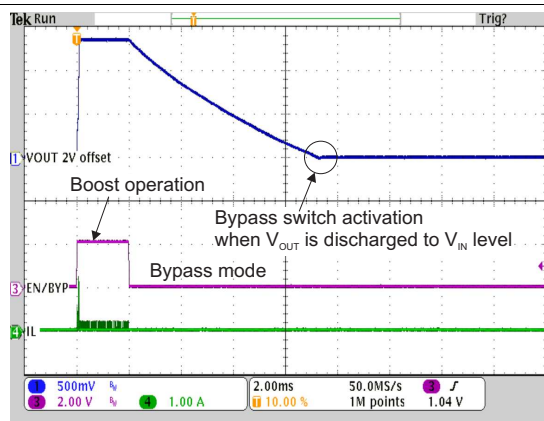
V_{IN} = 2.0V L = 3.3\mu H C_{OUT} = 22 \mu F V_{OUT} = 3.3V VSEL = GND R_{LOAD} = 1k\Omega
