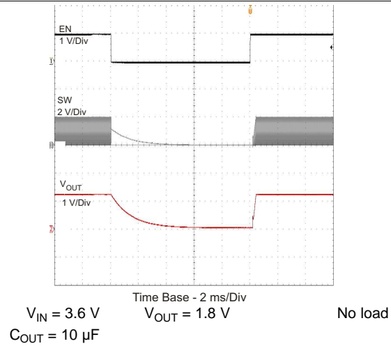
Figure 21. Output Discharge
