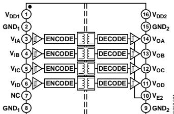
Figure 1. ADuM3400 Functional Block Diagram
