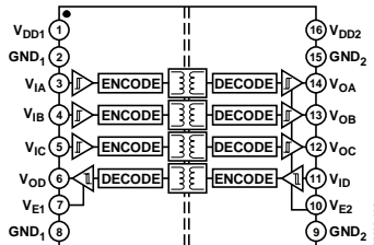
Figure 2. ADuM3401 Functional Block Diagram
