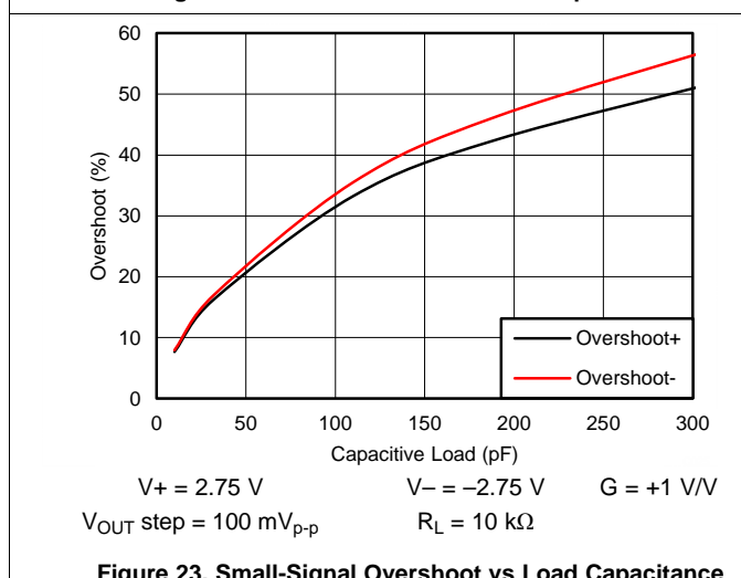
Figure 23. Small-Signal Overshoot vs Load Capacitance
