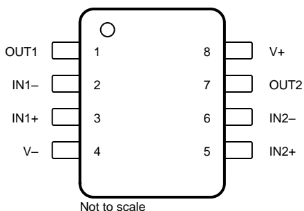
TLV9062 D, DGK, PW Packages 8-Pin SOIC, VSSOP, TSSOP Top View
