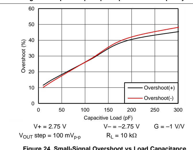
Figure 24. Small-Signal Overshoot vs Load Capacitance
