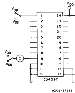
Fig. 7—OFF channel leakage current—any channel OFF.
