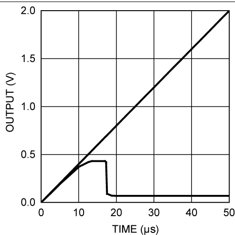
Figure 31. Power-On Reset
