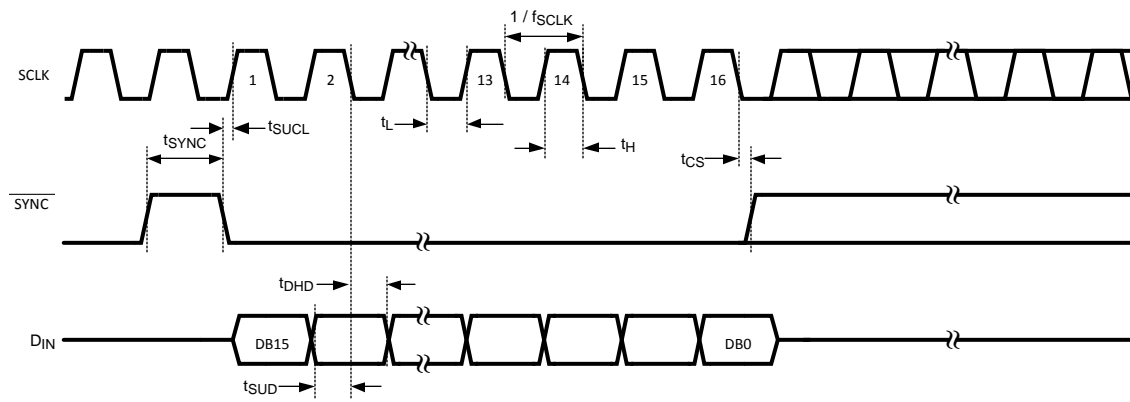
Figure 2. DAC121S101 Timing
