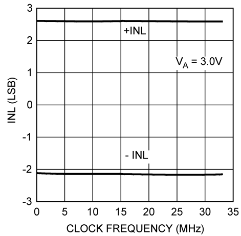
Figure 16. 3-V INL vs. f_{SCLK}
