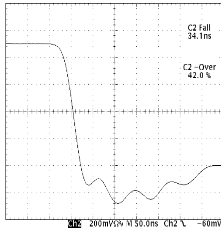
Figure 63. Fall Time
