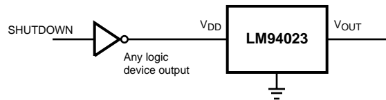
Figure 16. Conserving Power Dissipation with Shutdown
