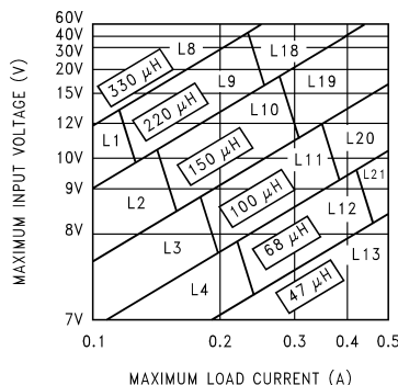
Figure 22. LM2594/LM2594HV-5.0
