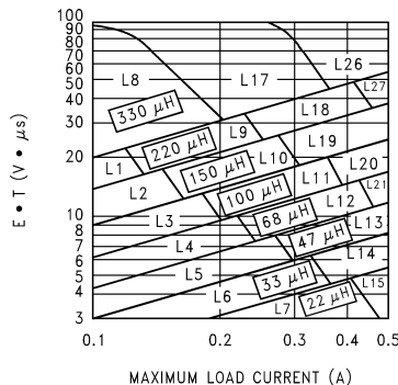
Figure 24. LM2594/LM2594HV-ADJ
