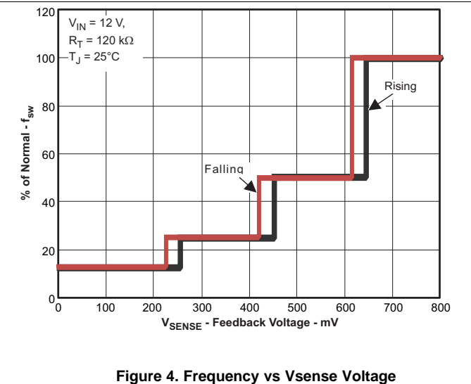
Figure 4. Frequency vs V_{sense} Voltage
