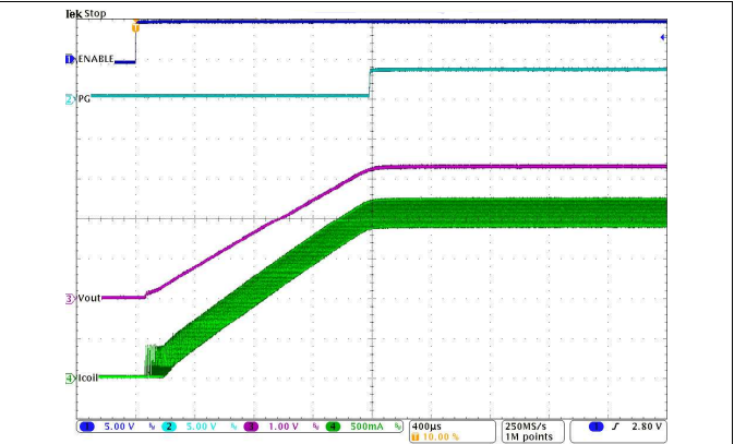
Figure 33. Startup into 3 A
