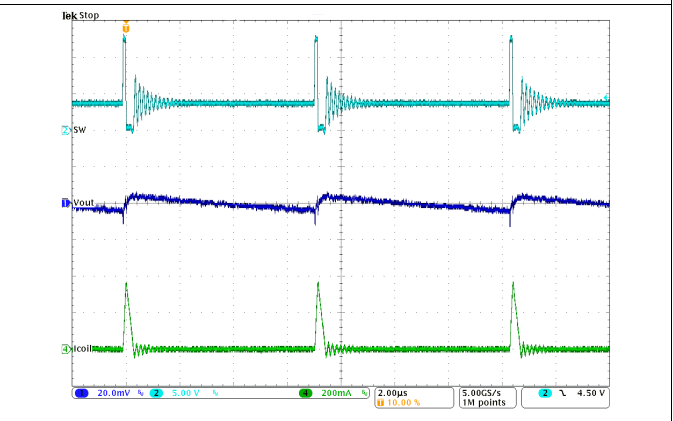
Figure 35. Typical Operation in Power Save Mode ( I_{OUT} = 10\text{ mA} )
