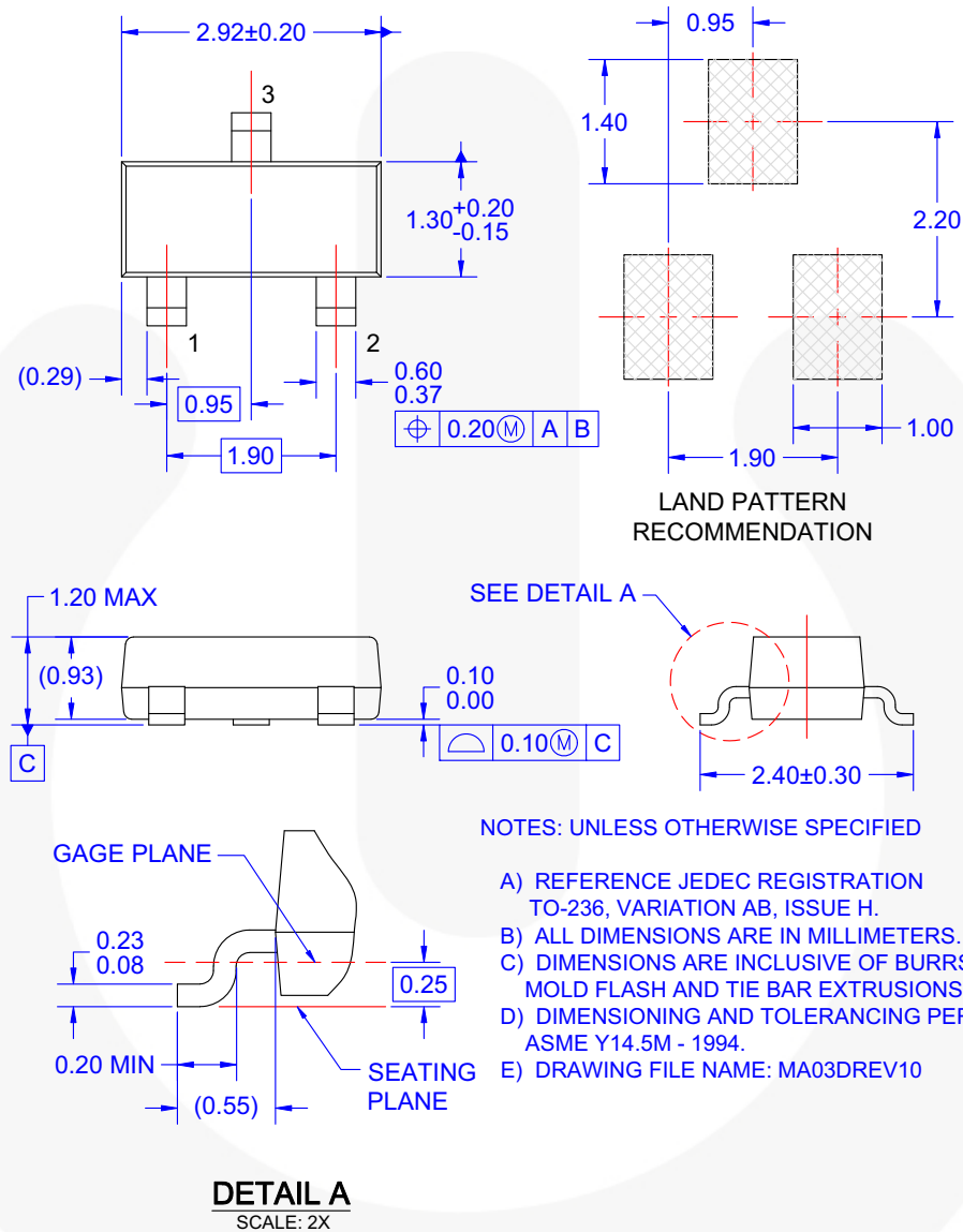
Figure 21. 3-LEAD, SOT23, JEDEC TO-236, LOW PROFILE
