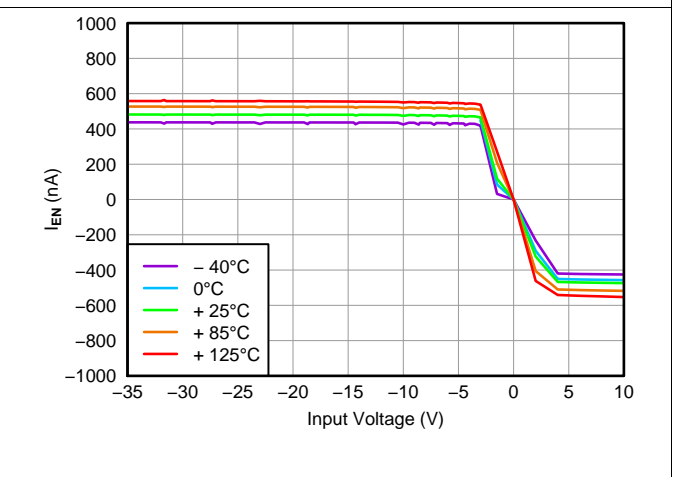
Figure 6. Enable Current vs Enable Voltage
