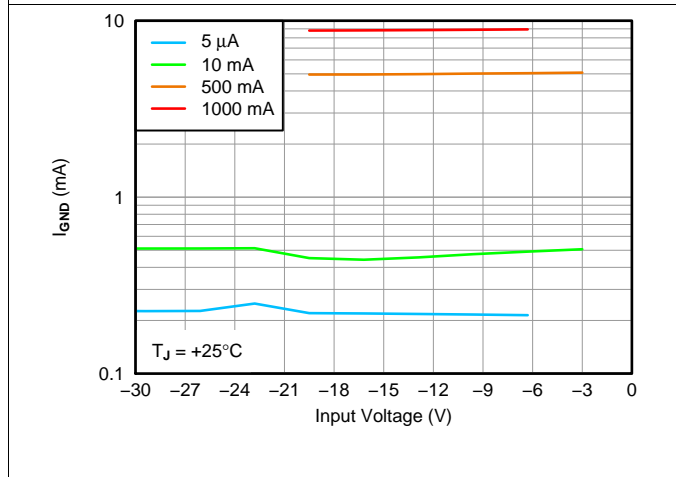
Figure 3. Ground Current vs Input Voltage
