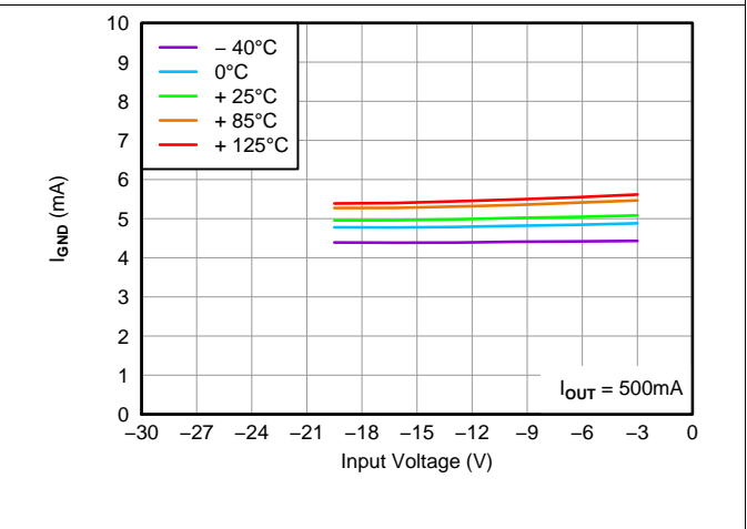
Figure 4. Ground Current vs Input Voltage
