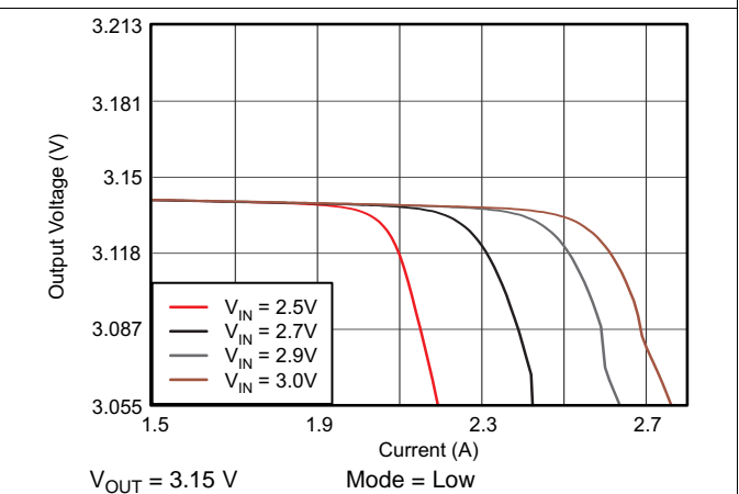
Figure 34. TPS61281A DC Output Voltage vs Output Current
