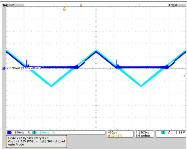
Figure 59. Boost to Pass-Through Mode Exit / Entry
