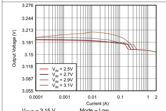
Figure 33. TPS61281A DC Output Voltage vs Output Current
