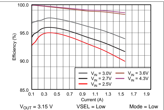
Figure 30. TPS61281A Efficiency vs Output Current
