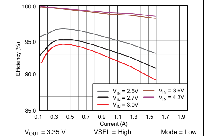
Figure 32. TPS61281A Efficiency vs Output Current
