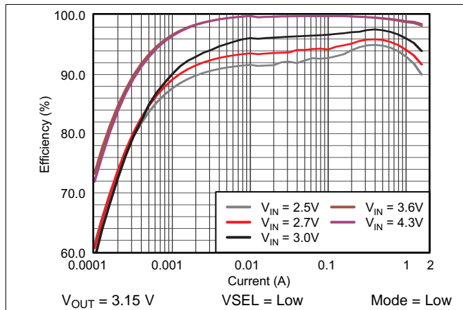
Figure 29. TPS61281A Efficiency vs Output Current
