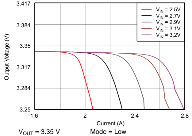
Figure 36. TPS61281A DC Output Voltage vs Output Current
