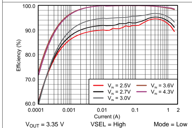
Figure 31. TPS61281A Efficiency vs Output Current
