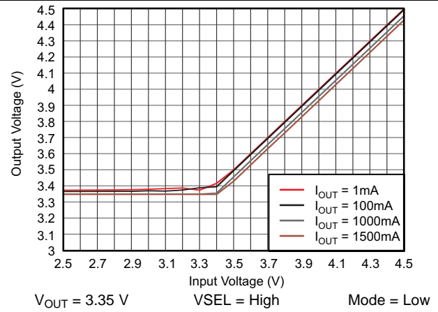
Figure 38. TPS61281A DC Output Voltage vs Input Voltage
