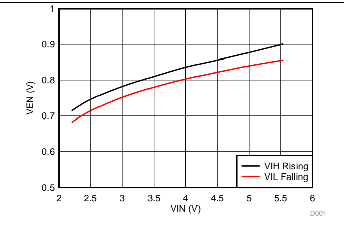
Figure 2. V_{EN} Thresholds vs V_{IN}
