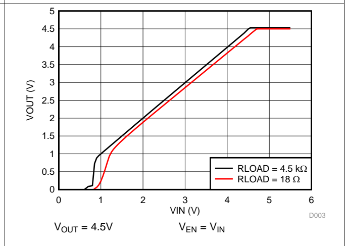
Figure 4. V_{OUT} vs V_{IN}
