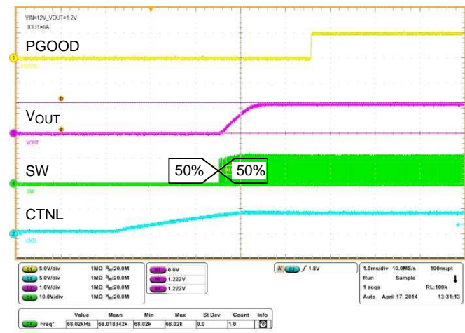
Figure 48. Start-Up Sequence
