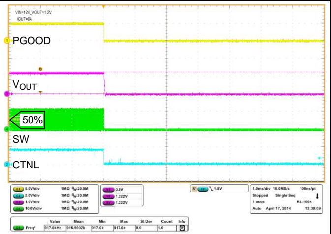
Figure 49. Shutdown Sequence
