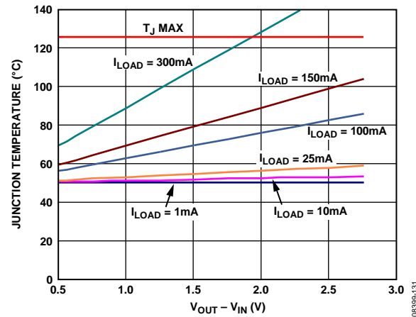
Figure 41. Junction Temperature vs. Power Dissipation, 500 mm 2 of PCB Copper, T A = 50°C
