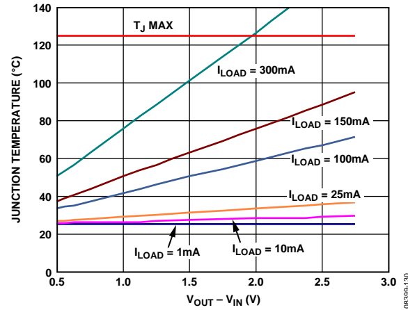
Figure 40. Junction Temperature vs. Power Dissipation, 0 mm 2 of PCB Copper, T A = 25°C
